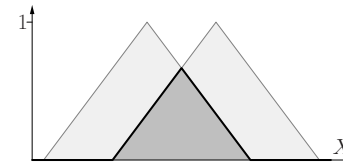
t -Norm T_{\min}
