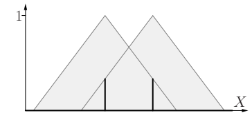
t -Norm T_{-1}
