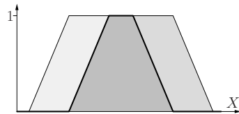
Fuzzy-Schnitt
