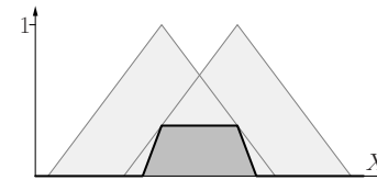
t -Norm T_{\text{Luka}}
