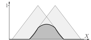
t -Norm T_{\text{prod}}
